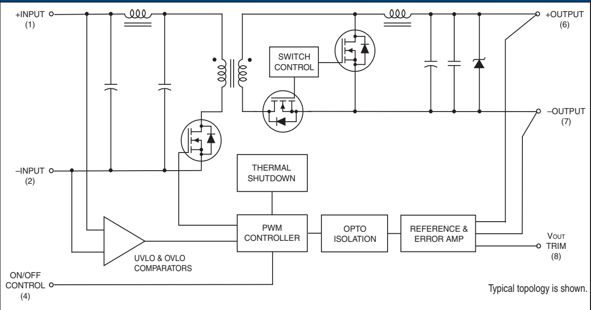
FIGURE 1. SIMPLIFIED SCHEMATIC
