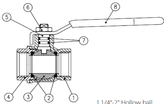
1.1/4"-2" Hollow ball
