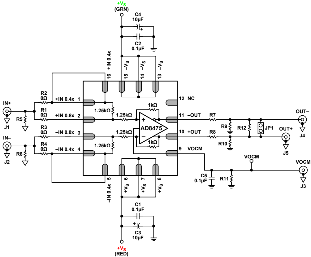
Figure 56. AD8475-EVALZ Schematic
