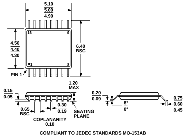
Figure 35. 16-Lead Thin Shrink Small Outline Package [TSSOP] (RU-16) Dimensions shown in millimeters
