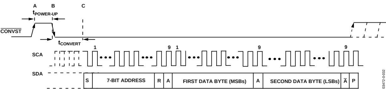
Figure 32. Mode 1 Operation
