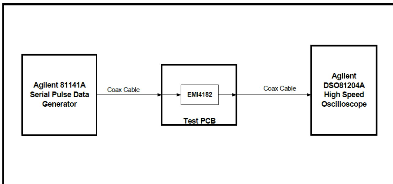
Figure 9. EMI4182 Eye Diagram Test Setup
