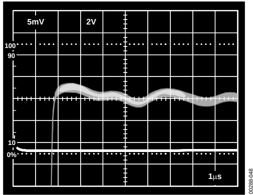
Figure 48. Positive Slope Settling Time
