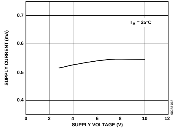
Figure 18. OP462 Supply Current/Amplifier vs. Supply Voltage
