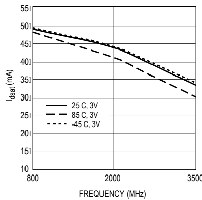
Figure 12. I_{dsat} vs. Frequency. □ ( P_{in} = 0 dBm, V_d = 3 V)
