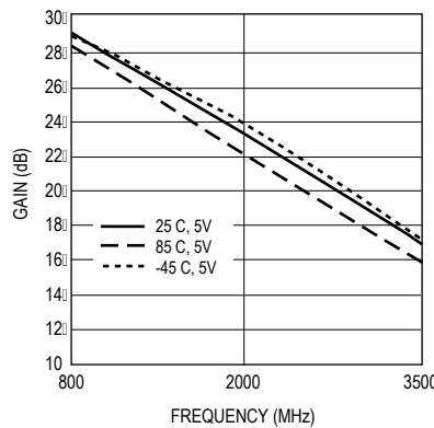
Figure 15. Gain vs. Frequency. □ ( P_{in} = -10 dBm, V_d = 5 V)
