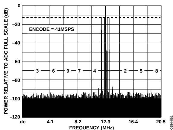
Figure 43. Multitone Performance
