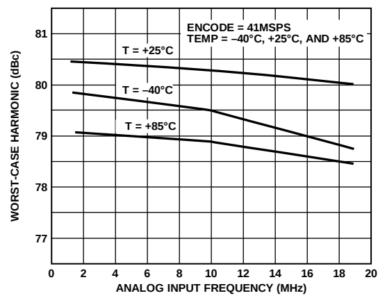
Figure 6. Worst-Case Harmonics vs. AIN
