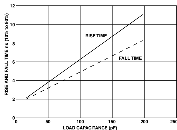
Figure 74. Typical Rise and Fall Times (10% to 90%) vs. Load Capacitance for Driver B at V_{DDEXT} = 2.25 V
