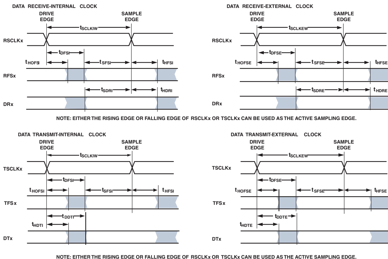
Figure 33. Serial Ports
