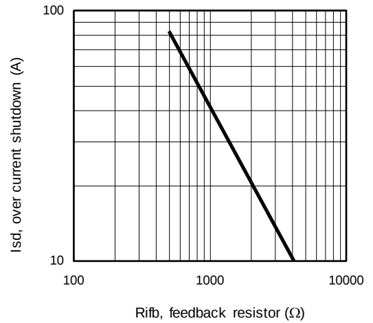
Figure 11 – Ids (A) Vs Rfcb (Ω)
