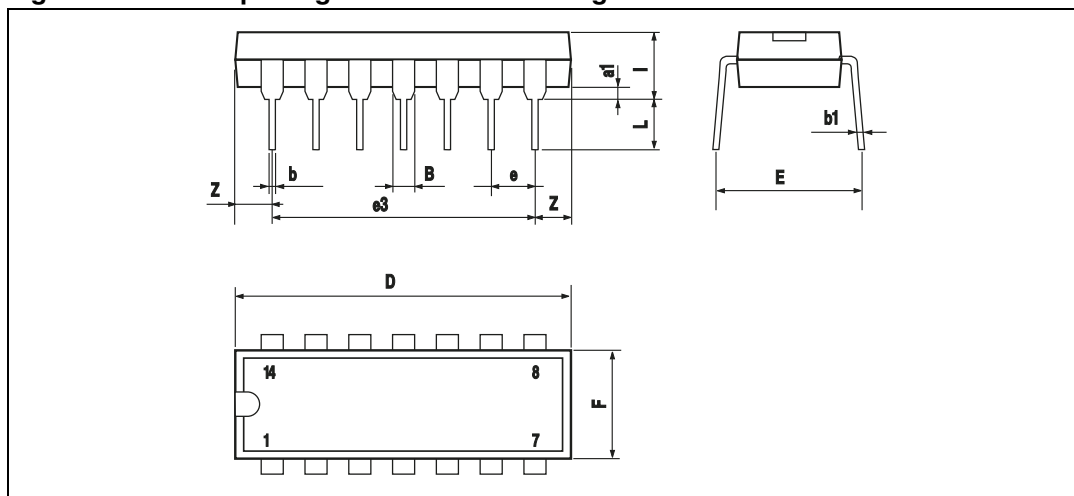
Figure 24. DIP14 package mechanical drawing
