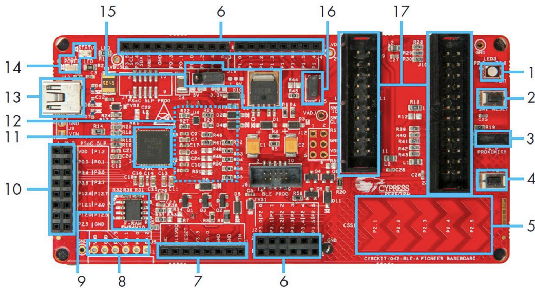
Figure 1-2. BLE Pioneer Baseboard
