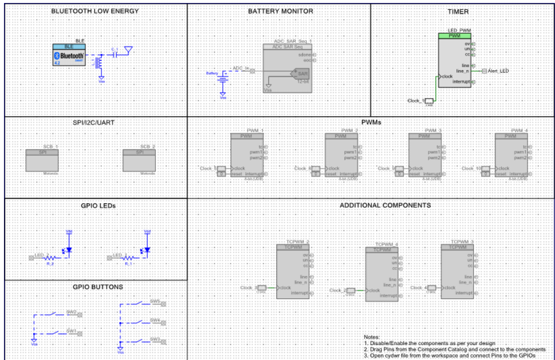
Figure 4-50. BLE_Dongle_Peripheral_IAS TopDesign
