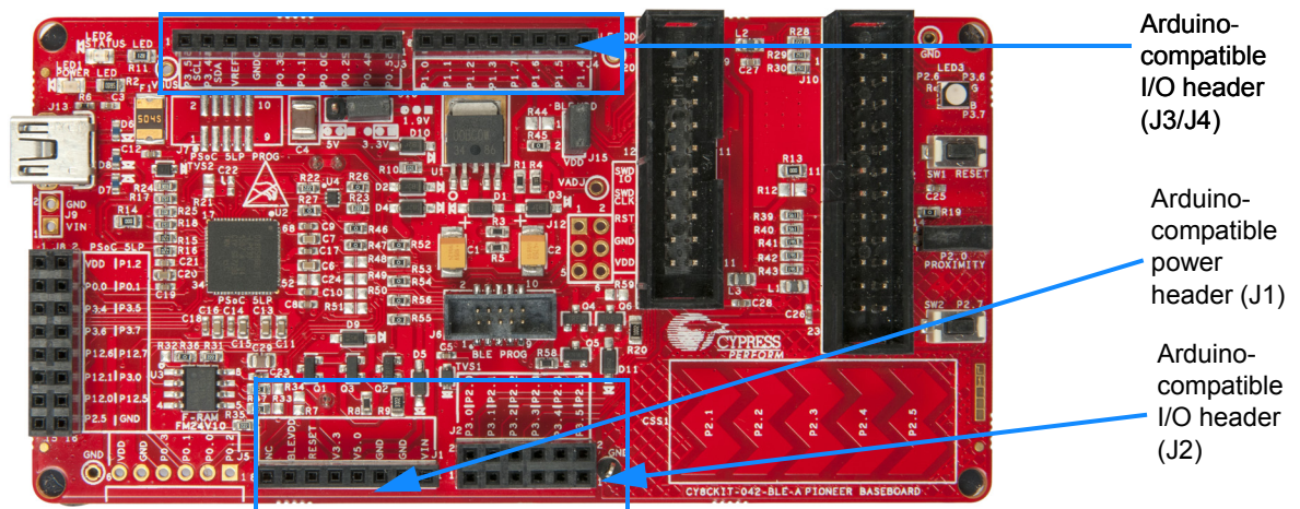
Figure 5-9. Arduino Headers
