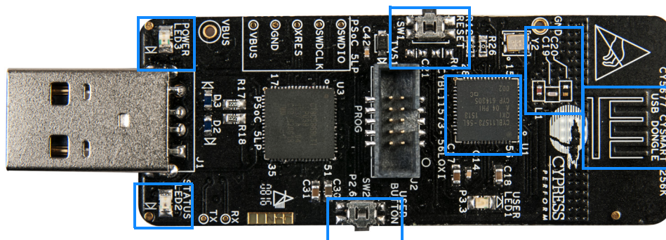
Figure 5-27. Board Highlight
