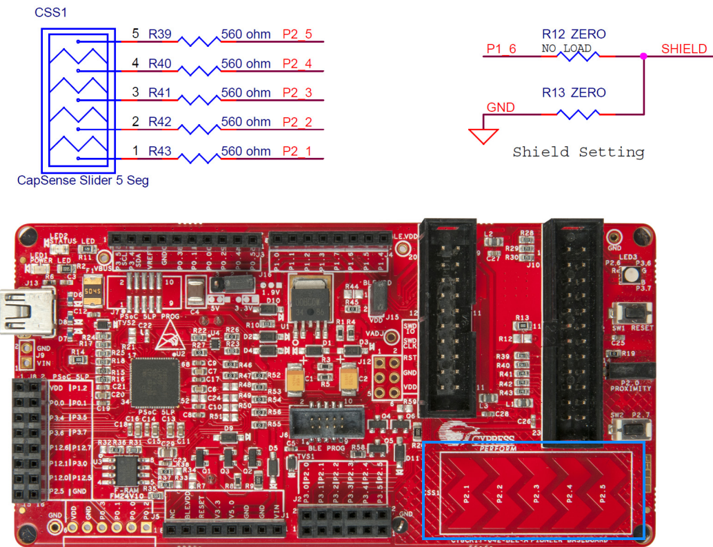
Figure 5-13. Schematics and Board Highlight of CapSense Slider and Shield Setting
