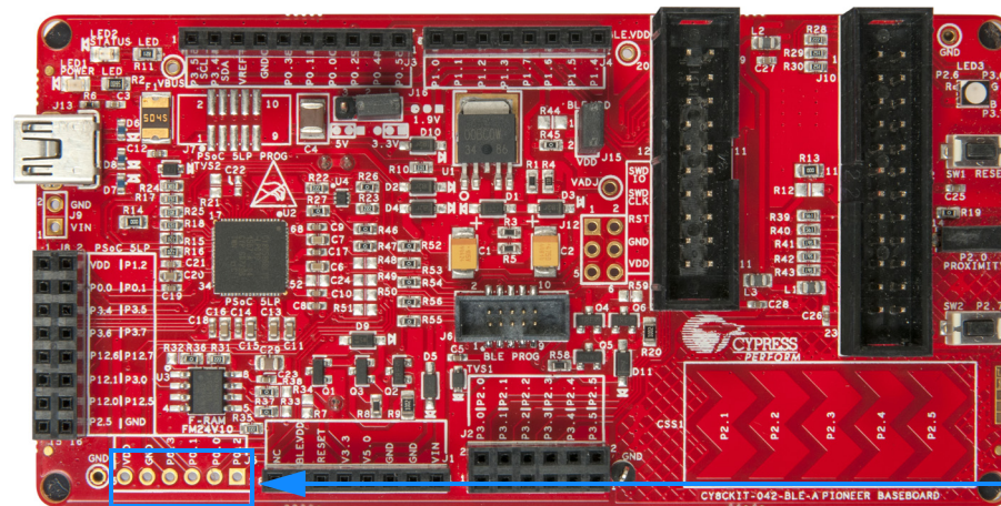
Figure 5-10. Schematics and Board Highlight of Pmod Connector
