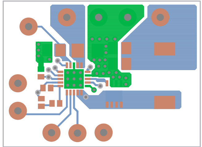
FIGURE 4. TOP LAYER
