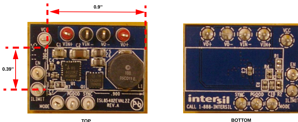
FIGURE 1. ISL85402EVAL2Z BOARD IMAGE
