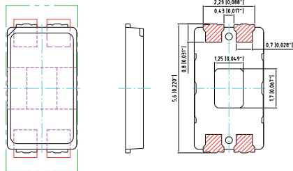
Component Location on Pad
