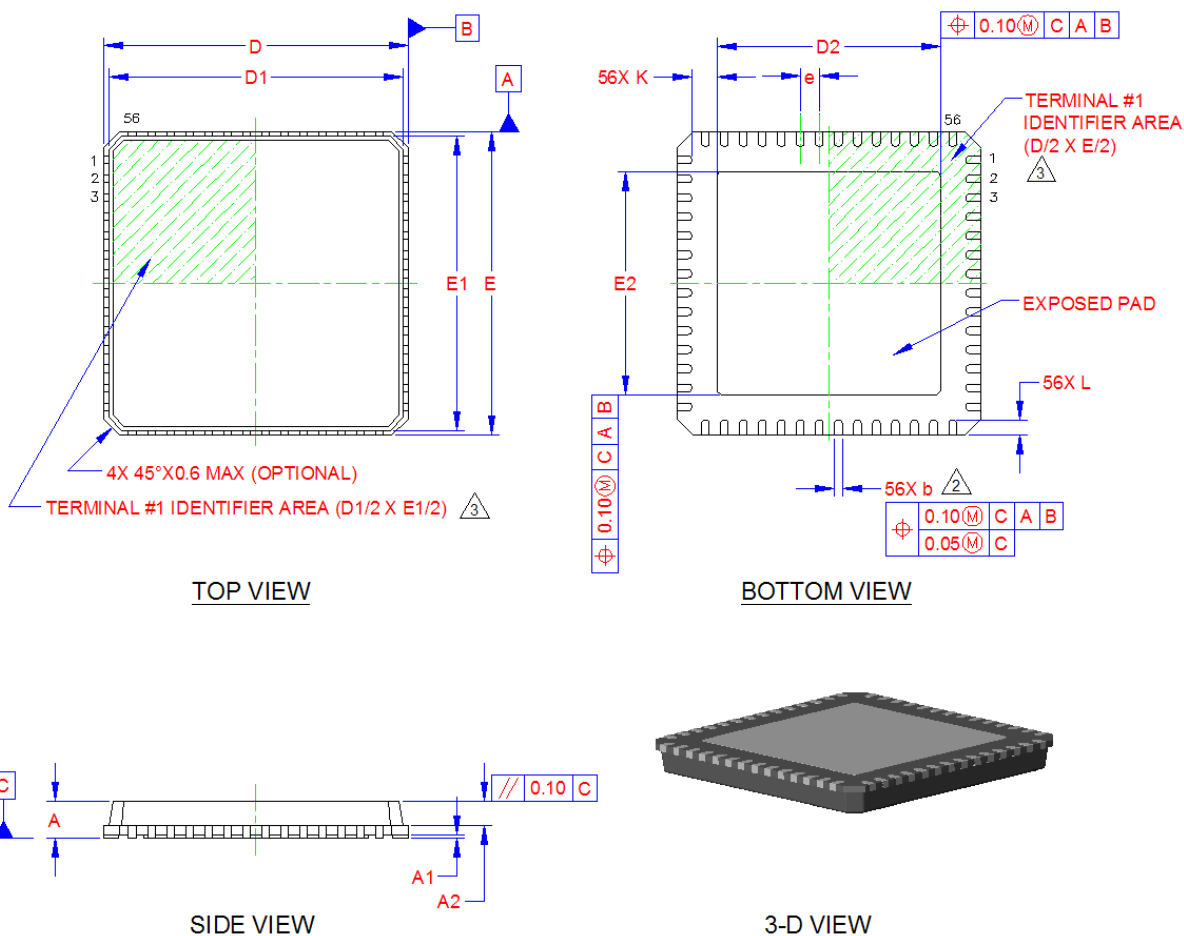
Figure 8.1 LAN7500/LAN7500i 56-QFN Package
