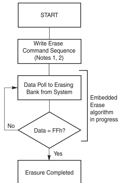
Figure 10.1 Erase Operation
