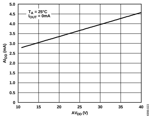
Figure 9. A_{1DD} vs. A_{V_{1DD}}
