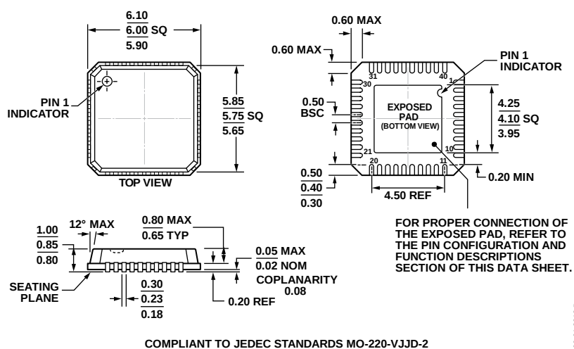
Figure 85. 40-Lead Lead Frame Chip Scale Package [LFCSP_VQ] 6 mm x 6 mm Body, Very Thin Quad (CP-40-1)
