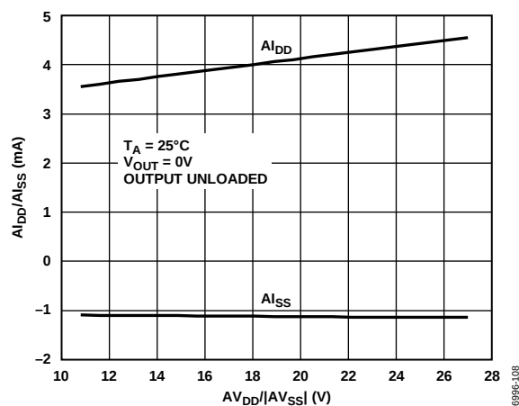
Figure 8. A_{1DD}/A_{1SS} vs. A_{V_{1DD}}/A_{V_{1SS}}
