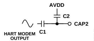
Figure 71. Coupling HART Signal
