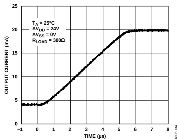
Figure 64. 4 mA to 20 mA Output Current Step
