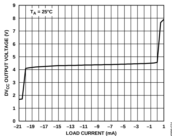
Figure 10. D_{V_{1CC}} Output Voltage vs. Load Current
