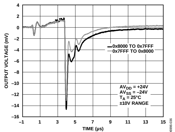
Figure 40. Digital-to-Analog Glitch
