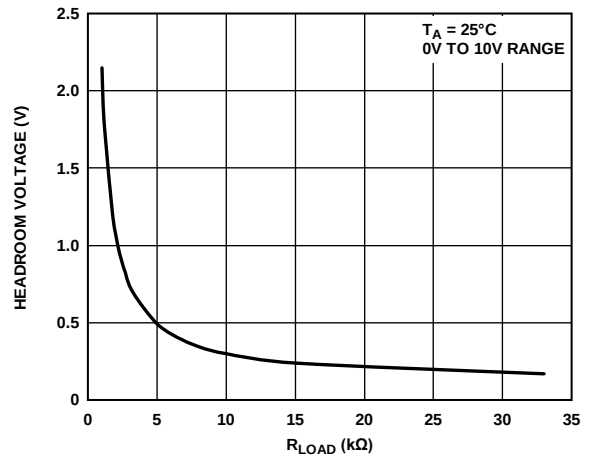
Figure 34. V_{OUT} Headroom
