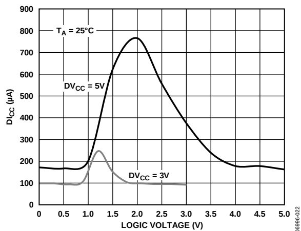
Figure 7. D_{1CC} vs. Logic Input Voltage
