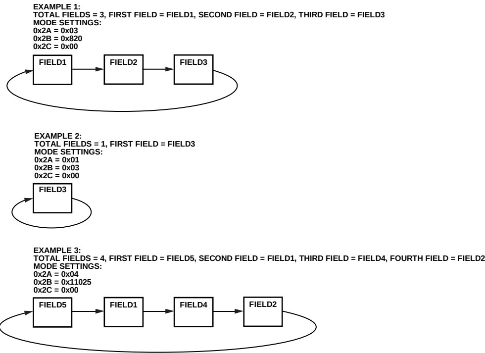
Figure 61. Using the Mode Registers to Select Field Timing
