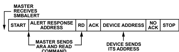
Figure 68. INT/INT Responds to SMBALERT ARA
