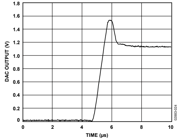
Figure 23. Exiting Power-Down to Midscale
