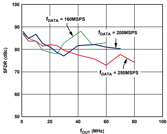
Figure 9. AD9779A In-Band SFDR vs. f_{OUT} , 2x Interpolation
