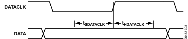
Figure 82. Input Data Port Timing, Data Referenced to DATACLK
