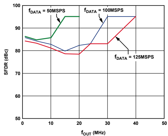
Figure 11. AD9779A In-Band SFDR vs. f_{OUT} , 8x Interpolation
