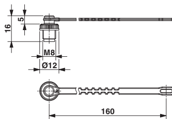
Dimensioned drawing
