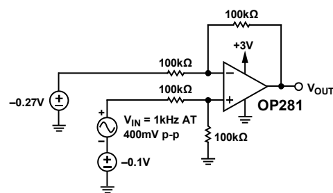
Figure 37. Single OPx81 Channel Configured as a Difference Amplifier Operating at V_{CM} \leq 0\text{ V}
