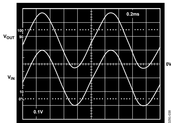
Figure 38. Input and Output Signals with V_{CM} < 0 V
