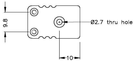
Miniature Hi-Temp Plastic in-line Socket - HTP (dimensions in mm)
