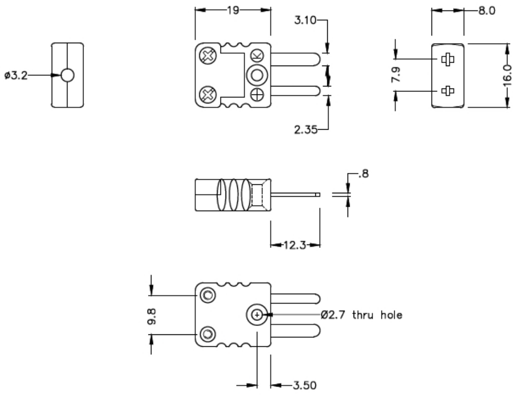
Miniature Hi-Temp Plastic in-line Plug - HTP (dimensions in mm)
