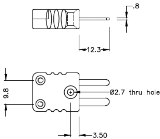
Miniature Hi-Temp Plastic in-line Plug - HTP (dimensions in mm)
