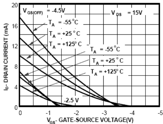
Transfer Characteristics
