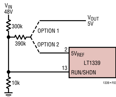
Figure 3. Input Supply Sequencing Programming
