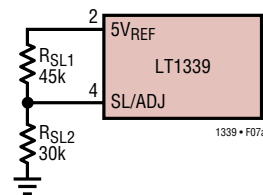
Figure 7a. External Slope Compensation Resistors
