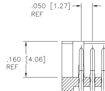
SECTION Y-Y
