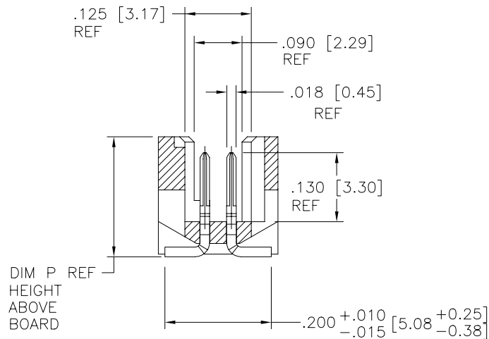
SECTION X-X ROTATED 90° CW
