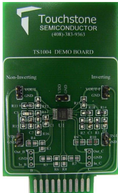
Figure 2. TS1004 Evaluation Board
