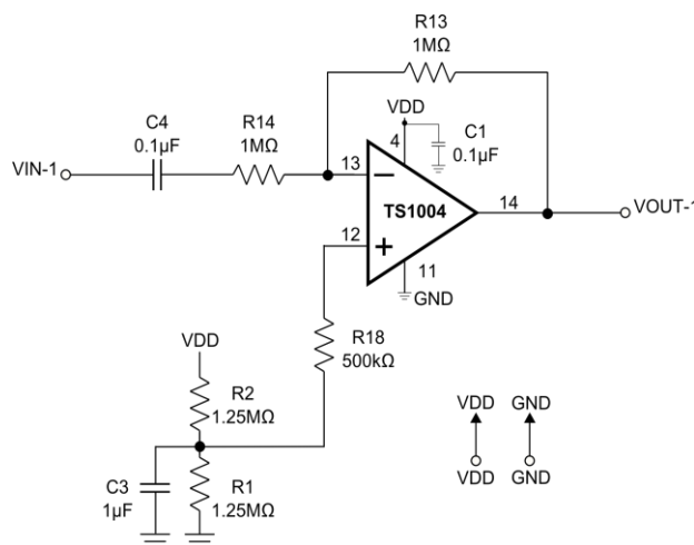
Figure 7. TS1004 Amp 'D' Inverting Configuration
