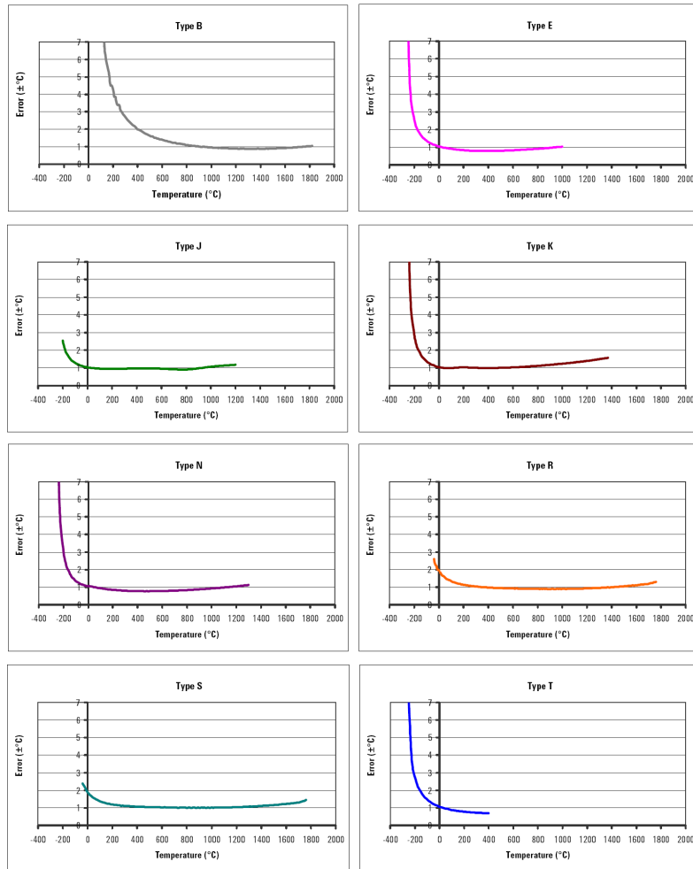
Figure 4-2 U2802A measurement accuracy plot for various thermocouples type
