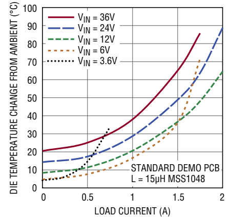
Die Temperature Rise vs Load Current, V_{OUT} = 5V , f_{SW} = 1.5\text{MHz}
