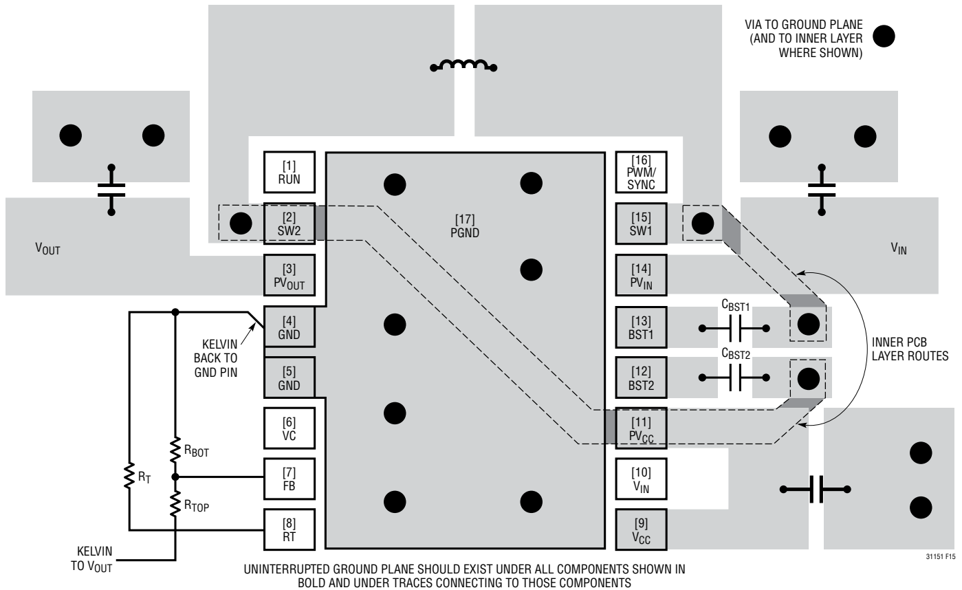
Figure 15. PCB Layout Recommended for the DHD Package
