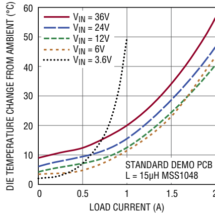
Die Temperature Rise vs Load Current, V_{OUT} = 5V , f_{SW} = 750\text{kHz}
