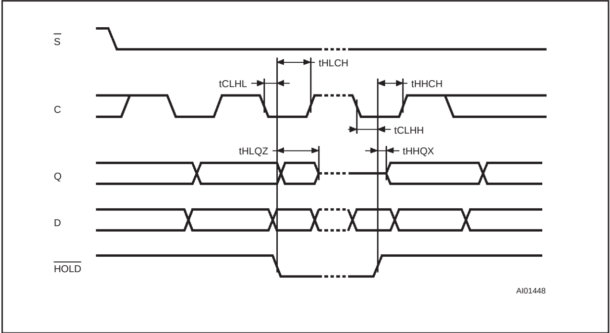
Figure 18. Hold Timing
