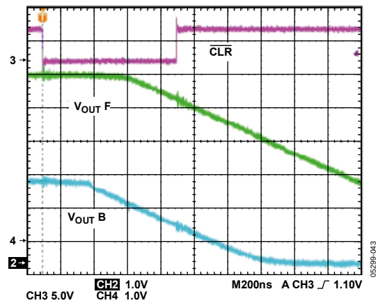
Figure 43. Hardware \overline{CLR}
