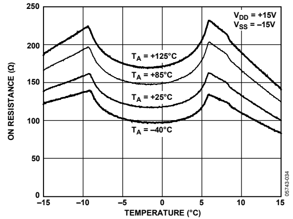
Figure 10. On Resistance as a Function of V_O ( V_S ) for Different Temperatures, Dual Supply
