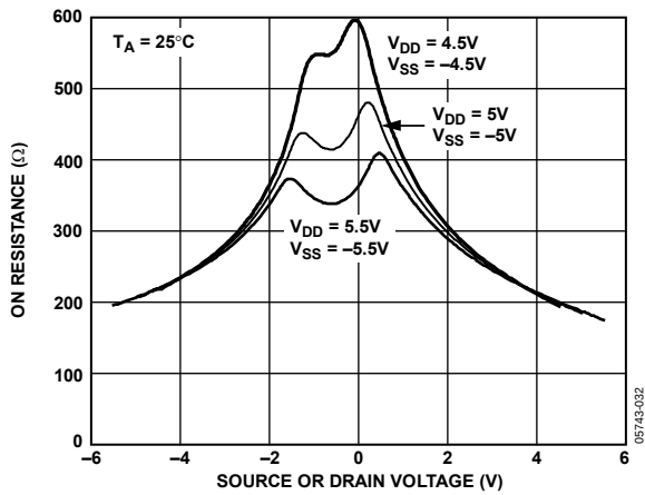
Figure 8. On Resistance as a Function of V_O ( V_S ) for Dual Supply
