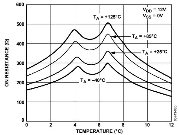
Figure 11. On Resistance as a Function of V_O ( V_S ) for Different Temperatures, Single Supply
