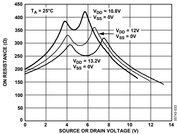
Figure 9. On Resistance as a Function of V_O ( V_S ) for Single Supply
