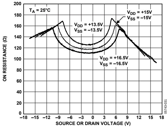
Figure 7. On Resistance as a Function of V_O ( V_S ) for Dual Supply
