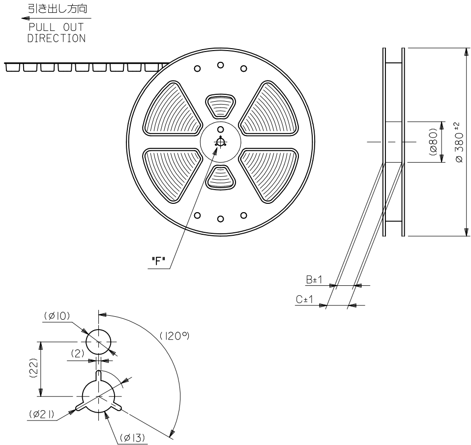
DETAIL "F"
