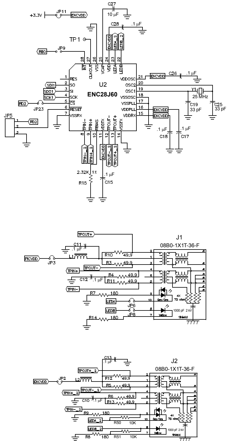
FIGURE A-3: PICDEM.net 2 DEVELOPMENT BOARD SCHEMATIC, SHEET 3 OF 5 (ENC28J60 INTERFACE AND ETHERNET MAGNETICS)
