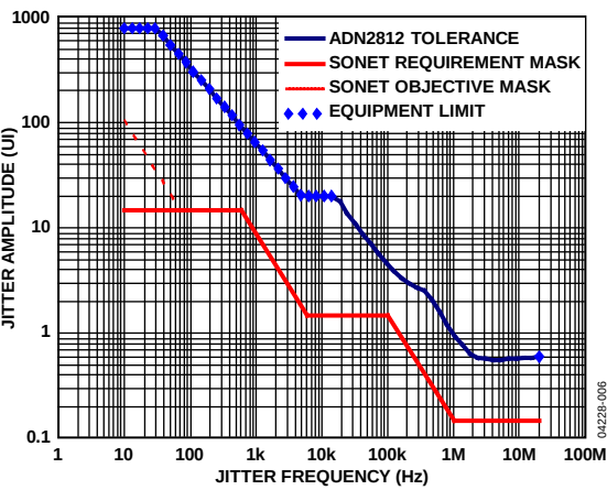
Figure 6. Typical Measured Jitter Tolerance OC-48
