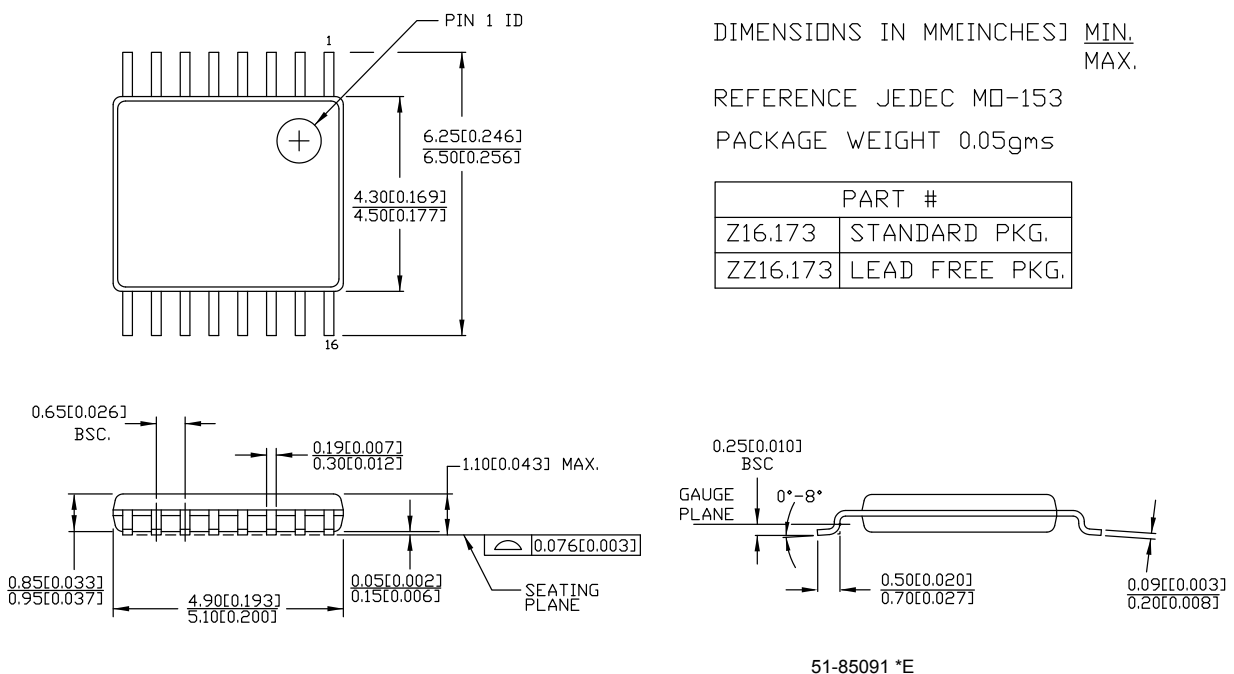
Figure 18. 16-pin TSSOP (4.40 mm Body) Z16.173/ZZ16.173 Package Outline, 51-85091
