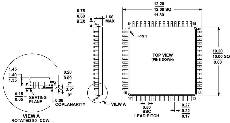
Figure 79. 64-Lead Low Profile Quad Flat Package [LQFP] (ST-64-2) Dimensions shown in millimeters
