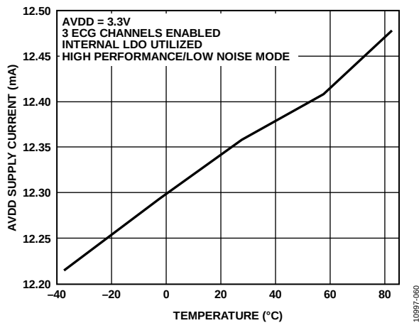
Figure 30. Typical AVDD Supply Current vs. Temperature, Using Internal ADVCC/DVDD Supplies
