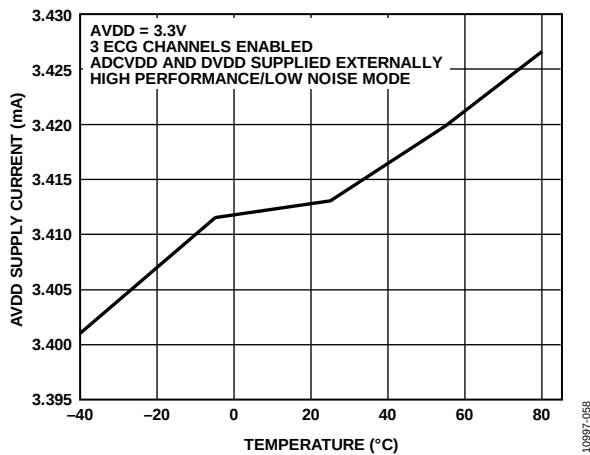
Figure 31. Typical AVDD Supply Current vs. Temperature, Using Externally Supplied ADVCC/DVDD
