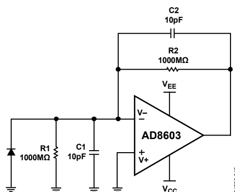
Figure 47. Photodiode Circuit
