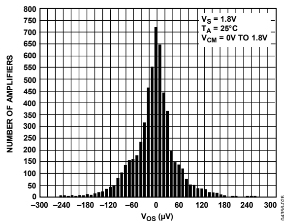
Figure 28. V_{OS} Distribution
