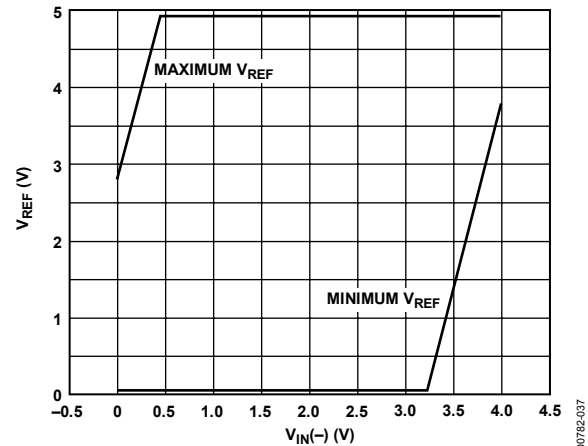
Figure 39. Reference Input Voltage vs. Negative Input Voltage, V_S = 5 \text{ V} , G = +5
