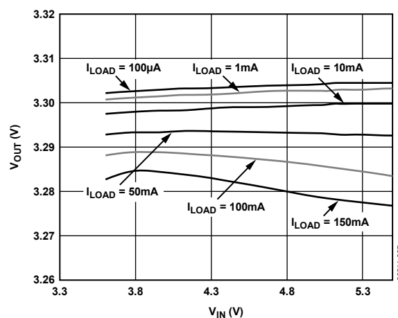
Figure 6. ADP1710 Line Regulation
