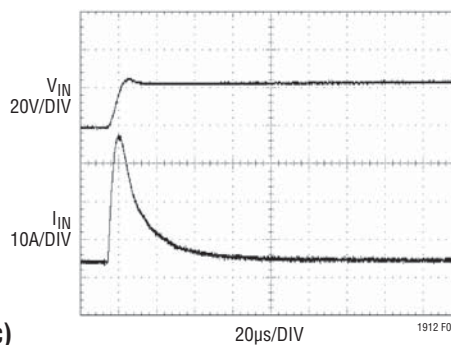
Figure 9. A Well Chosen Input Network Prevents Input Voltage Overshoot and Ensures Reliable Operation when the LT1912 is Connected to a Live Supply
