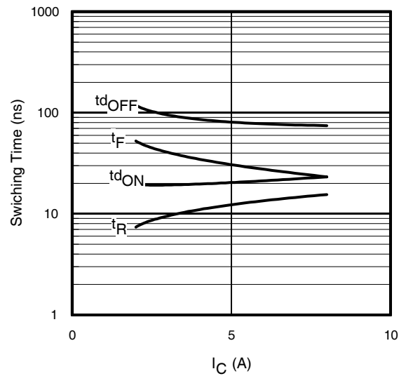
Fig. 14 - Typ. Switching Time vs. I_C
