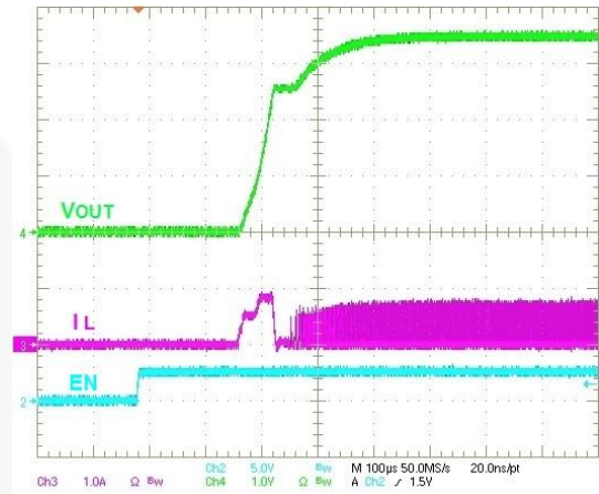
Figure 18. Startup, 50 Ω Load, V_{IN} = 2.6\text{ V} , V_{OUT} = 3.5\text{ V}
