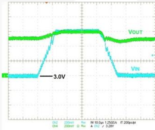
Figure 25. Line Transient, 3.0-3.6 V_{IN} , 10 \mu\text{s} Edge, 500 mA Load, V_{OUT}=3.5\text{ V}
