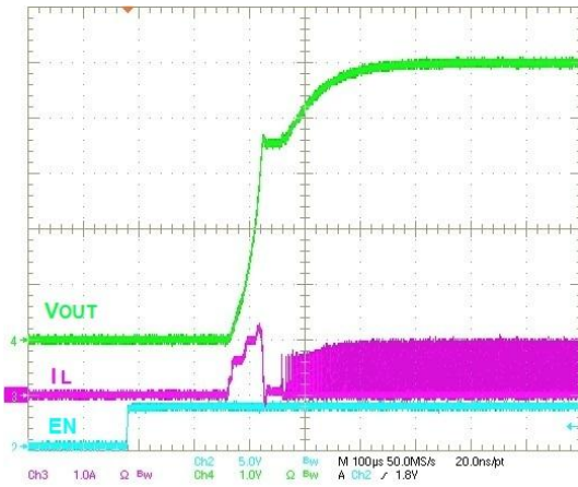
Figure 17. Startup, 50 Ω Load
