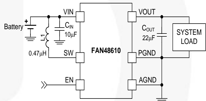
Figure 1. Typical Application
