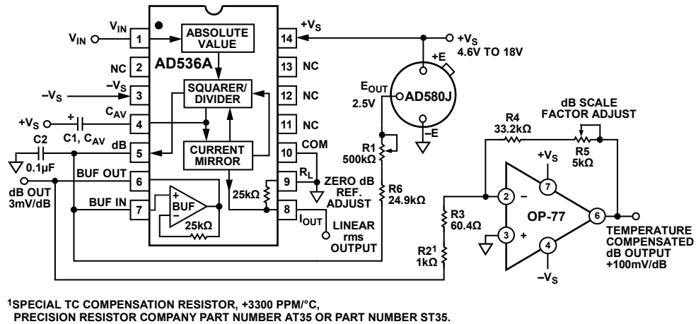
Figure 17. dB Connection
