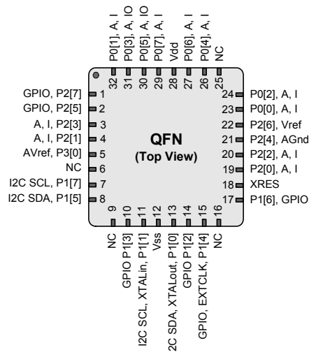
Figure 3. CY8C23533 32-Pin PSoC Device
