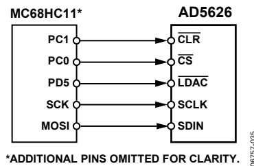
Figure 35. AD5626 to MC68HC11 Interface
