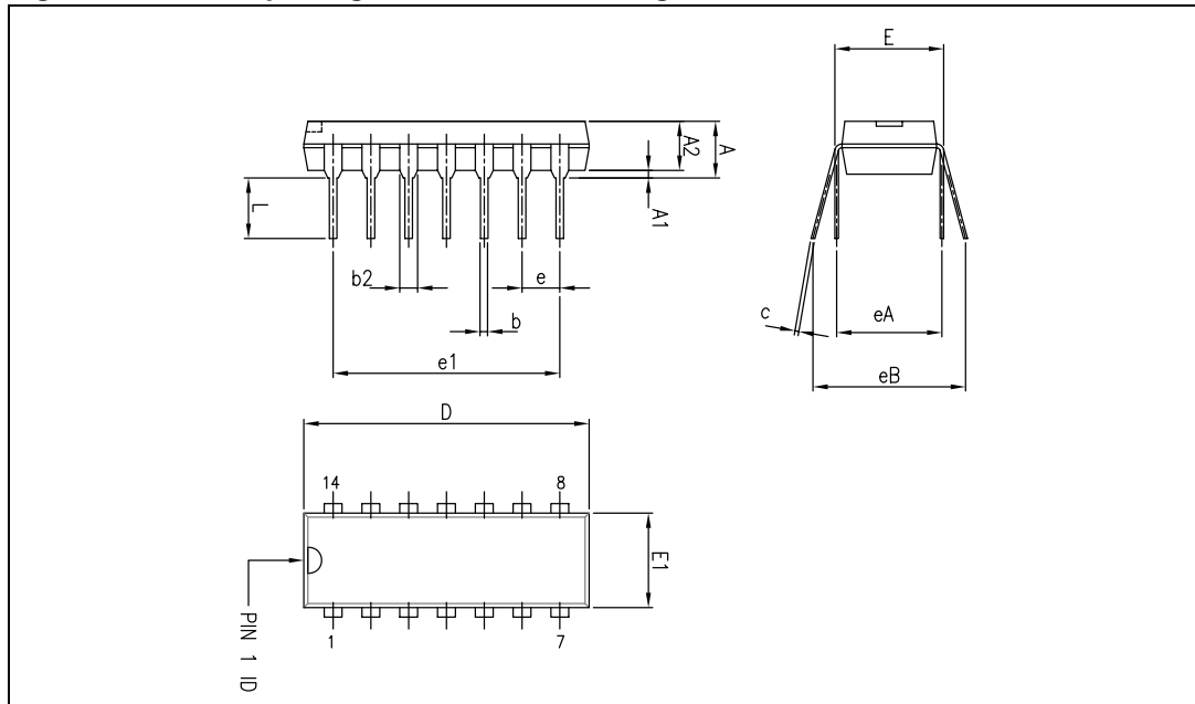
Figure 21. DIP14 package mechanical drawing
