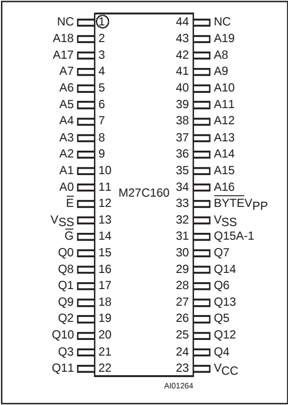
Figure 4. SO Connections
