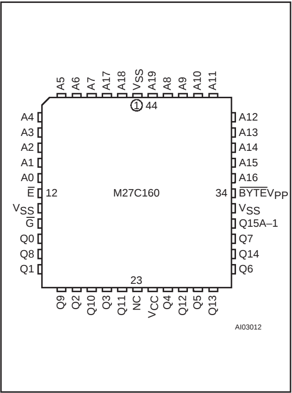
Figure 3. PLCC Connections
