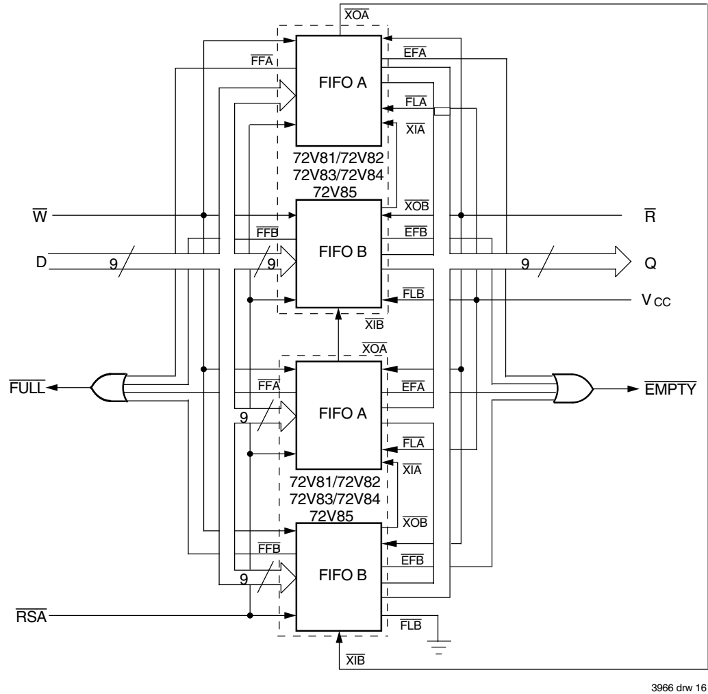
Figure 14. Block Diagram of 2,048 x 9, 4,096 x 9, 8,192 x 9, 16,384 x 9 and 32,768 x 9 FIFO Memory (Depth Expansion)
