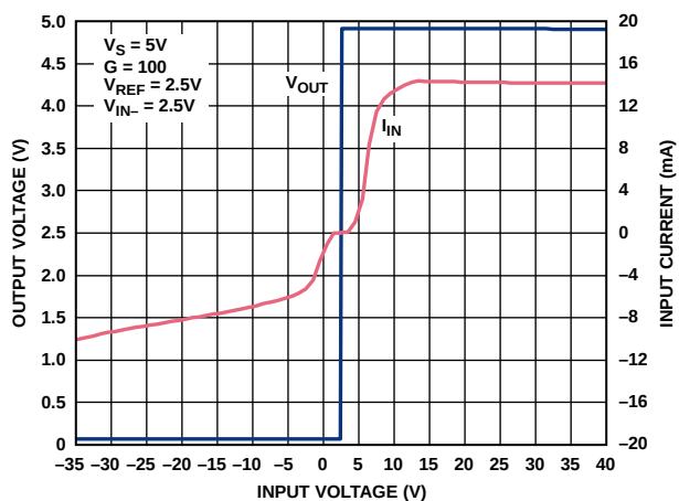
Figure 18. Input Overvoltage Performance; G = 100 , V_S = 5\text{ V}
