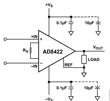
Figure 60. Supply Decoupling, REF, and Output Referred to Local Ground
