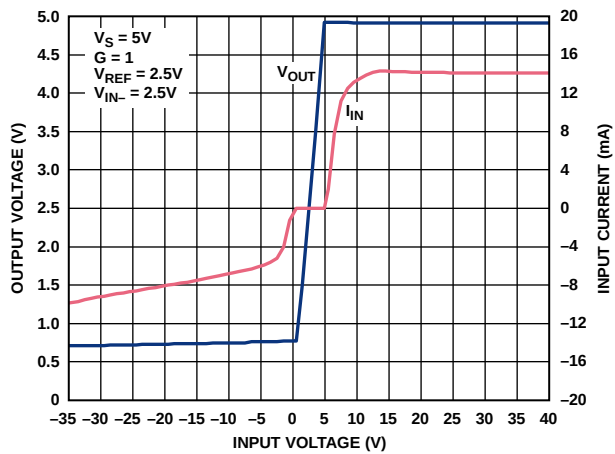
Figure 16. Input Overvoltage Performance; G = 1 , V_S = 5\text{ V}
