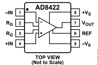
Figure 59. Pinout Diagram
