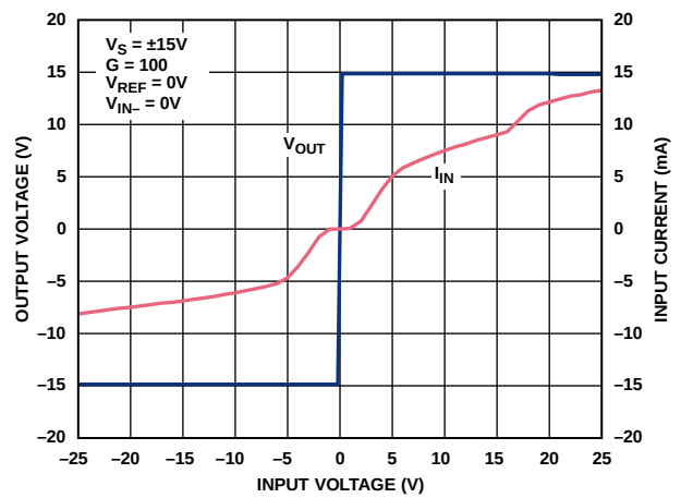
Figure 19. Input Overvoltage Performance; G = 100 , V_S = \pm 15\text{ V}
