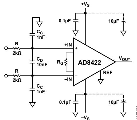
Figure 64. RFI Suppression
