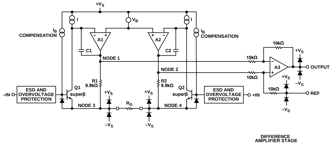
Figure 57. Simplified Schematic
