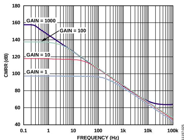
Figure 26. CMRR vs. Frequency, 1 k \Omega Source Imbalance
